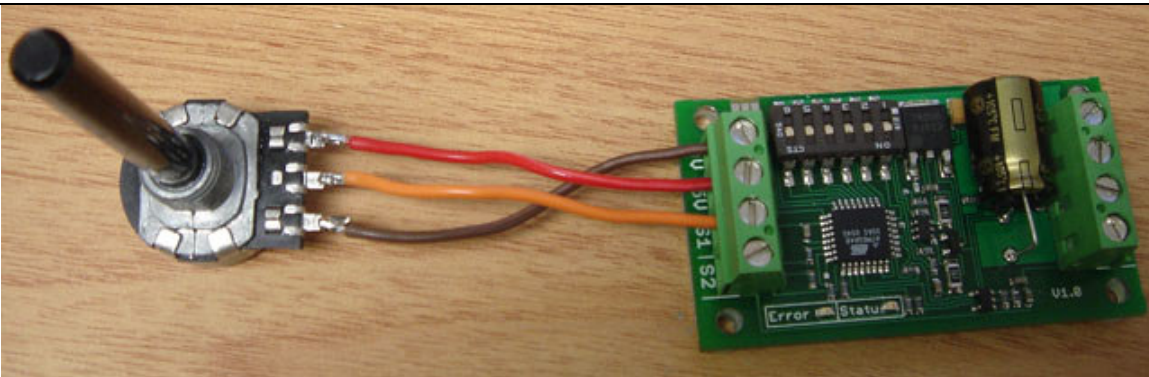
Figure 2.1: Analog input using a potentiometer powered from terminal 5V
