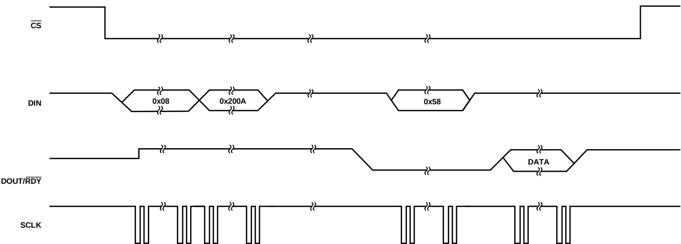
Figure 14. Single Conversion
