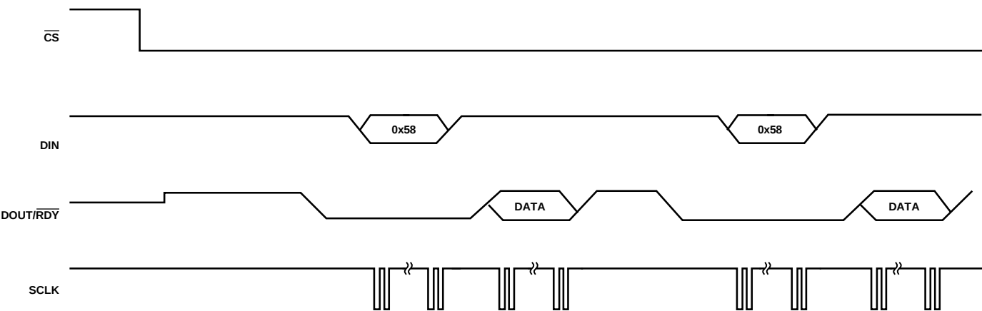
Figure 15. Continuous Conversion
