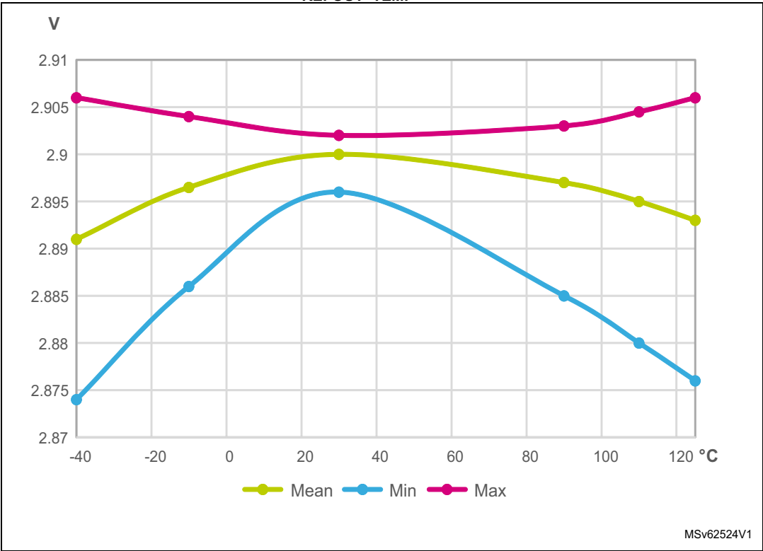
Figure 32. V_{\text{REFOUT}} TEMP in case VRS = 10
