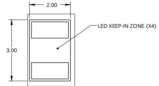
DETAIL F SCALE 10 : 1
