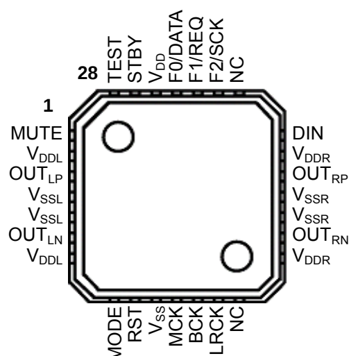
QFN28
