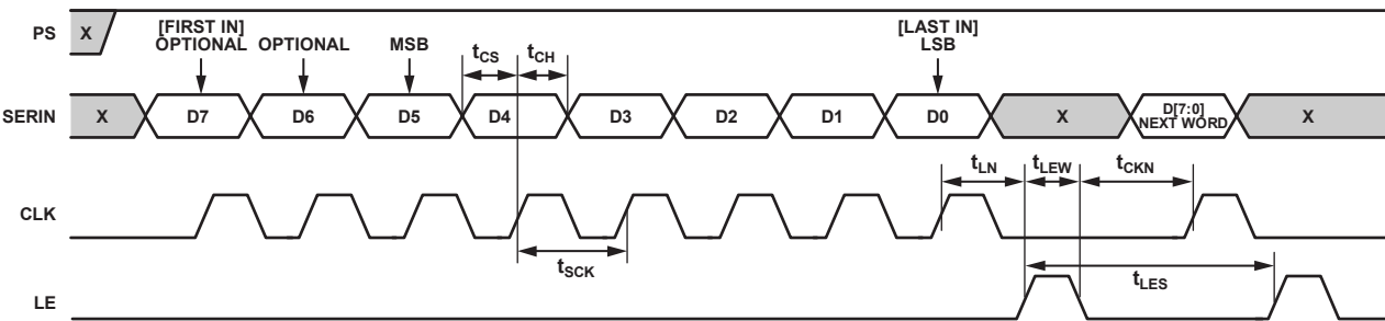
Figure 34. Serial Control Timing Diagram
