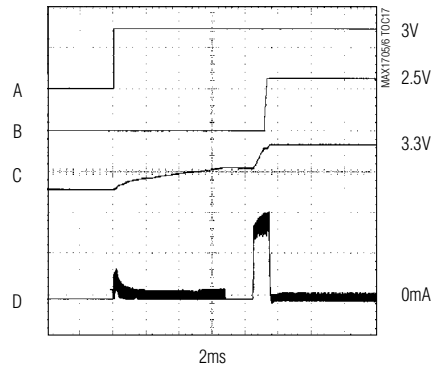
MAX1705 POWER-ON DELAY (PWM MODE)
