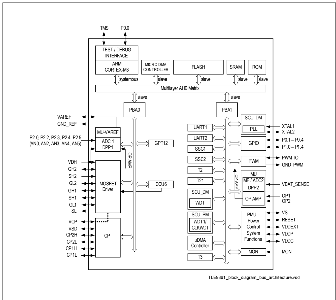
Figure 1 Block Diagram
