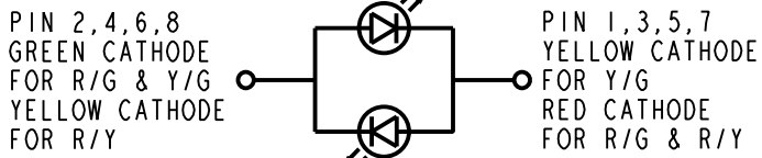
BI-COLOR LED SCHEMATIC
