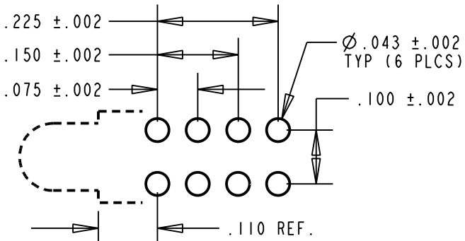
RECOMMENDED HOLE PATTERN
