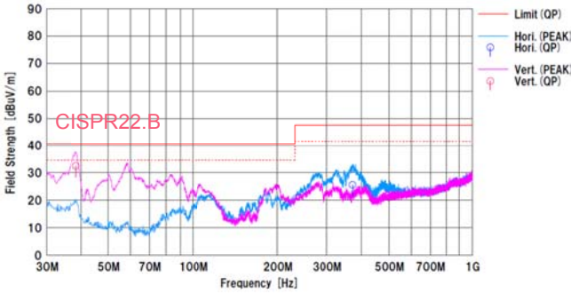
Figure 24. Radiated Emission.2 V IN =230Vac/50Hz, I OUT =0.5A QP margin= 8.0dB, AV margin=10.4dB
