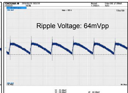
Figure 20. VOUT Ripple Voltage.6 V_{IN}=230Vac , I_{OUT}=500mA CH1: VOUT 50mV/div, 10µs/div
