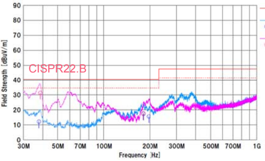
Figure 23. Radiated Emission.1 V IN =110Vac/60Hz, I OUT =0.5A QP margin=9.2dB, AV margin=11.2dB
