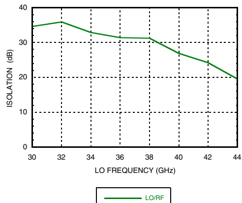
LO/RF isolation
