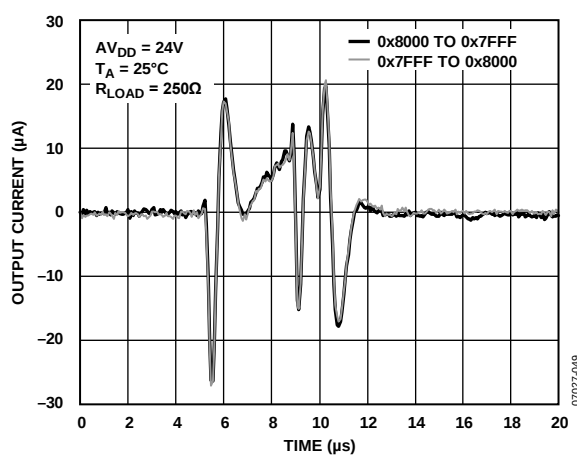
Figure 35. Digital-to-Analog Glitch
