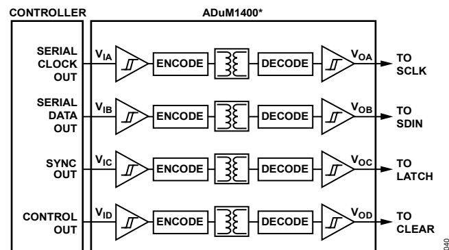
Figure 52. Isolated Interface
