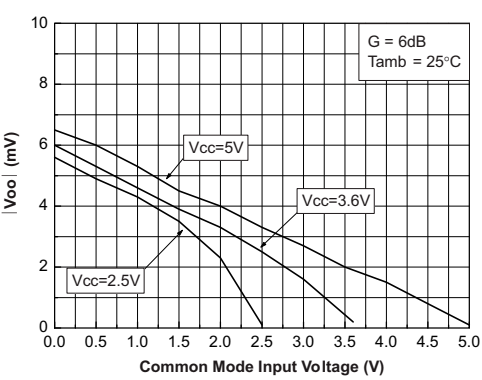
Figure 9. Output offset voltage vs. common-mode input voltage
