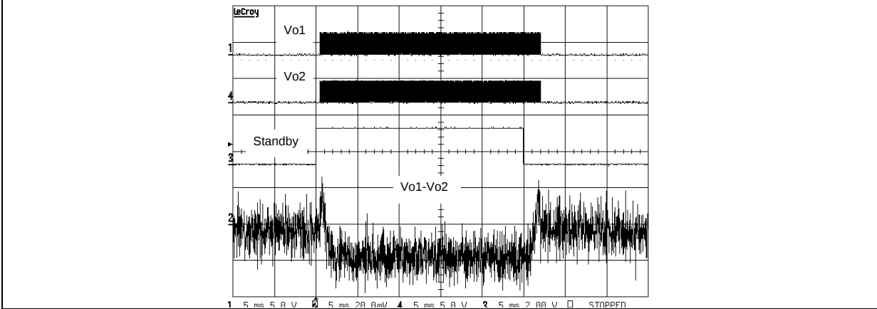
Figure 62. Startup and shutdown time V_{CC} = 3\text{ V} , G = 6\text{ dB} , no C_{in} (5 ms/div)
