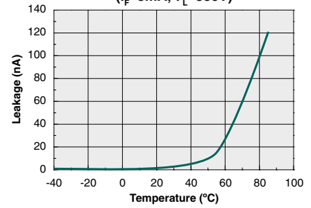
Leakage Current vs. Temperature Measured Across Pins 7 & 8 ( I_F=5mA, V_L=350V )
