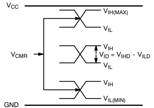
Figure 8. V_{CM} Diagram
