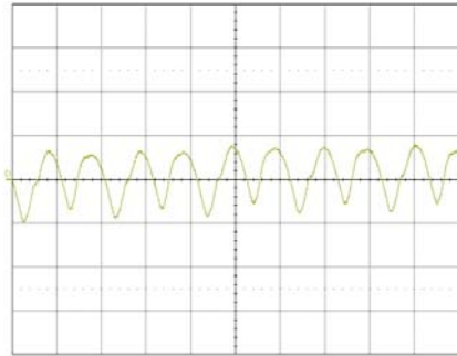
Output voltage ripple at: T_{ref} = +25^{\circ}C , V_I = 12 V , I_O = 30 A resistive load. Trace: output voltage (5 mV/div.). Time scale: (2 μs/div.).
