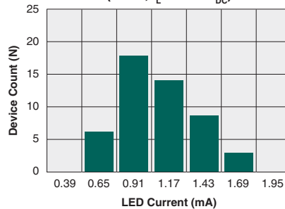
Typical I L for Switch Dropout (N=50, I L =120mA DC )
