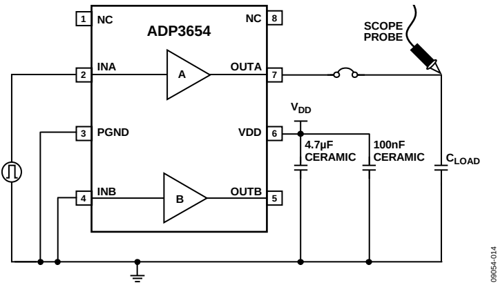
Figure 14. Test Circuit
