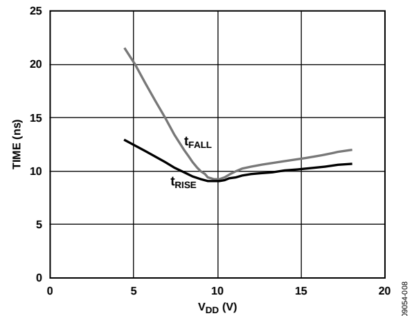
Figure 8. Rise and Fall Times vs. V_{DD}
