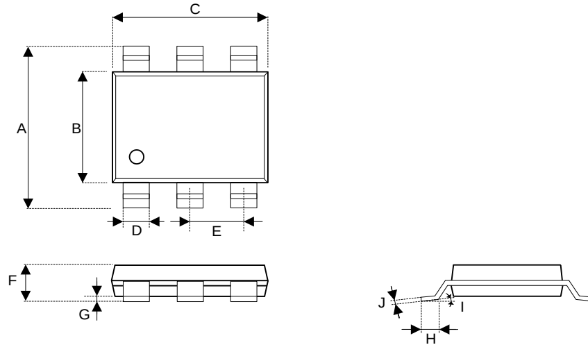
Figure 12.1 TSOT23-6 Packaging 5
