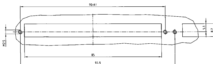
Panel cutout
