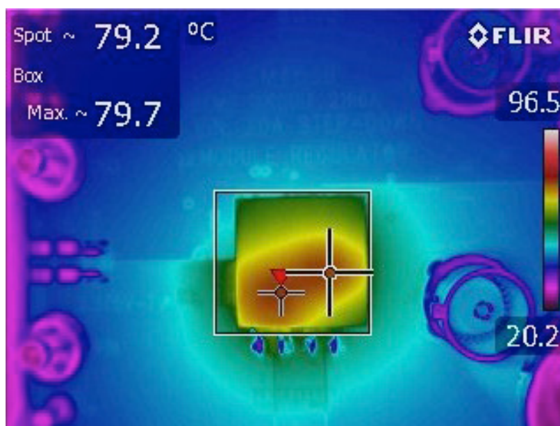
Figure 5. Thermal Image of LTM4639 V_{IN} = 3.3V , V_{OUT} = 1.8V , I_{LOAD} = 20A Ambient Temperature = 23.3^{\circ}C , No Forced Air Flow
