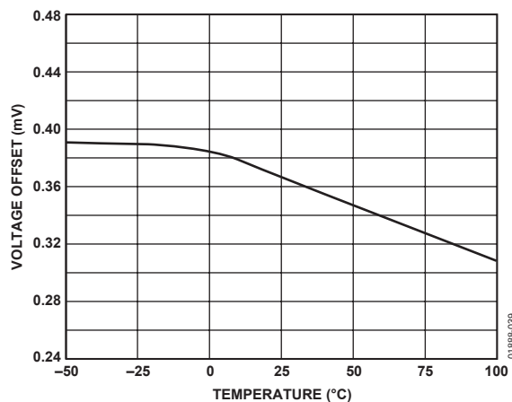
Figure 39. V_{\text{os}} vs. Temperature
