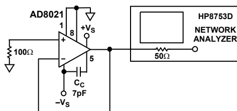
Figure 55. Output Impedance, Chip Disabled
