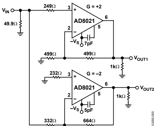
Figure 65. Differential Amplifier
