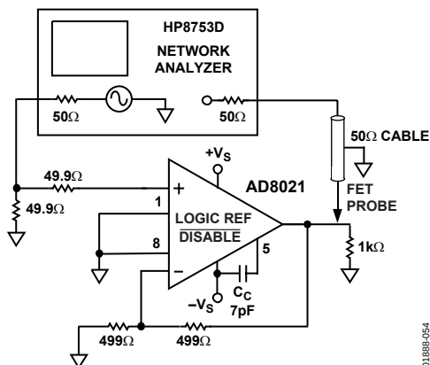
Figure 54. Input-to-Output Isolation, Chip Disabled
