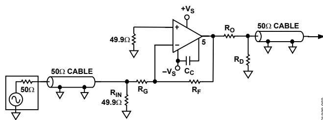
Figure 50. Inverting Gain
