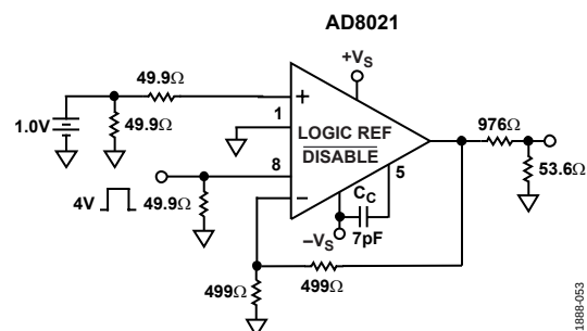
Figure 53. Enable/Disable
