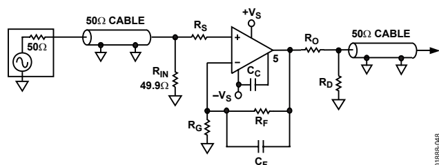
Figure 48. Noninverting Gain
