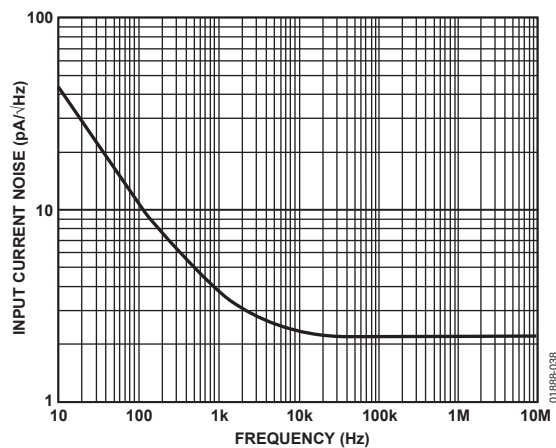
Figure 38. Input Current Noise vs. Frequency
