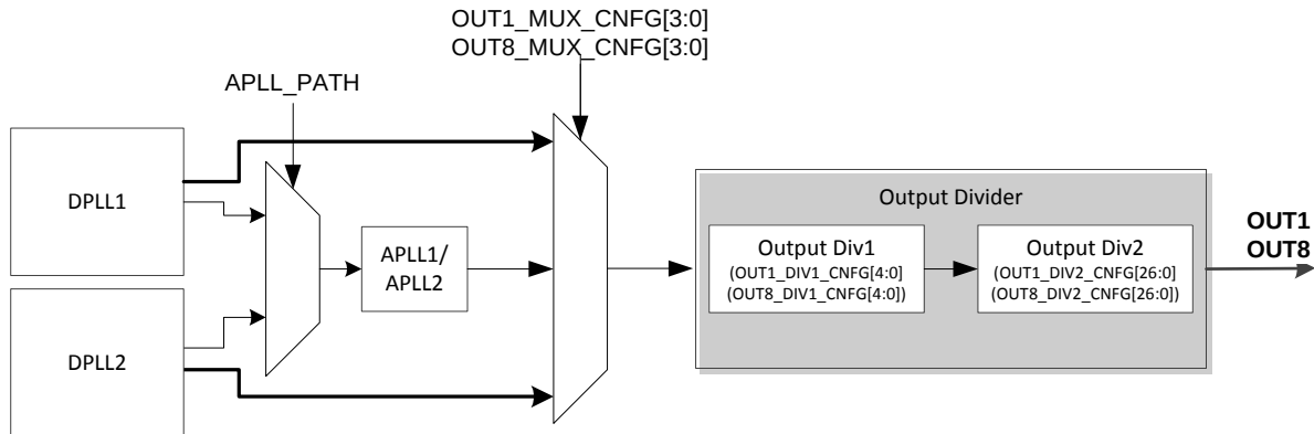
Figure 11. OUT1 and OUT8 output dividers
