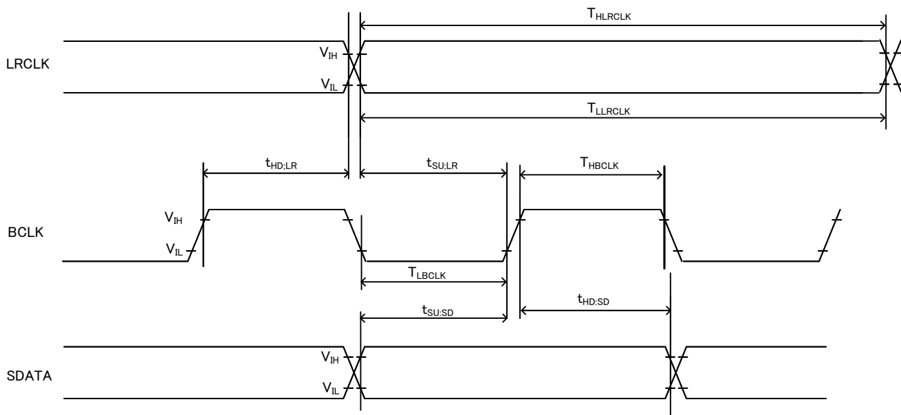
Figure 41. Clock timing
