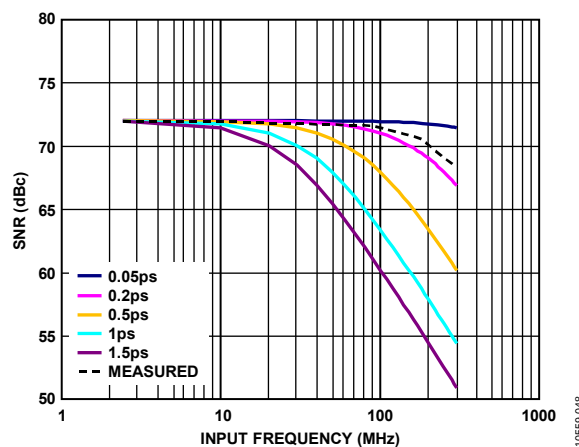
Figure 52. AD9250-250 SNR vs. Input Frequency and Jitter
