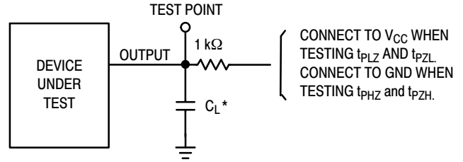
Figure 4. Test Circuit
