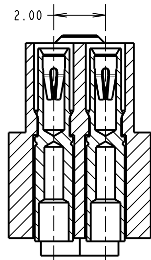
SECTION X-X
