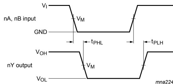
Figure 5. The input (nA and nB) to output (nY) propagation delays
