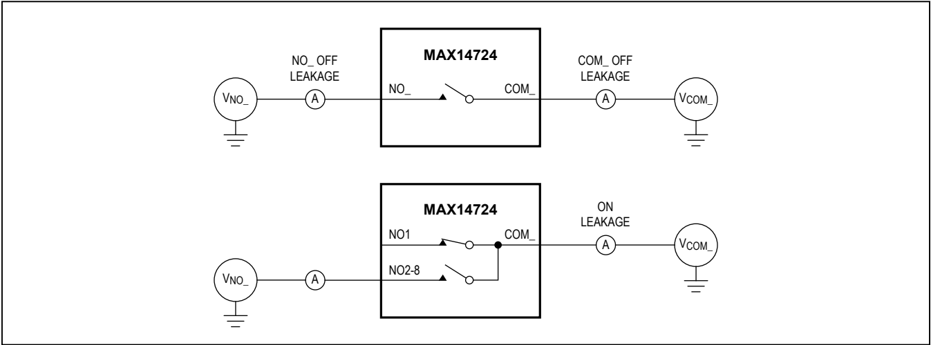
Figure 1. On/Off-Leakage Current
