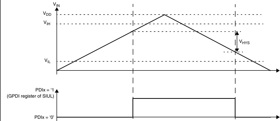
Figure 6. I/O input DC electrical characteristics definition
