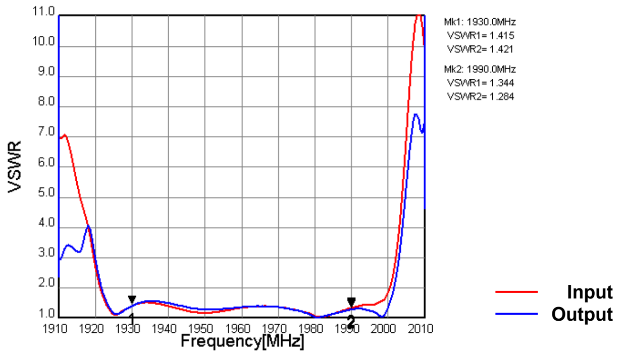
Fig.10 VSWR (Filter2)
