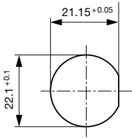
Drilling diagram
