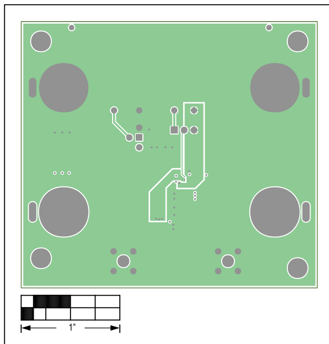
MAX17250 WLP EV Kit—Level 3 POWER
