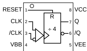
TOP VIEW 8-Pin MLF®
