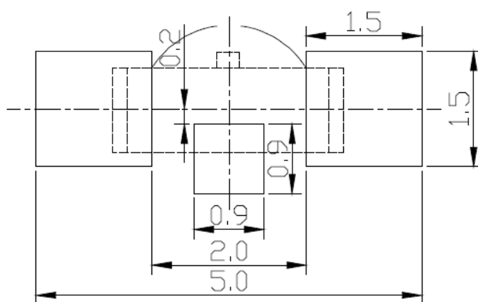
Figure 1. IN-S126AS Solder Pattern
