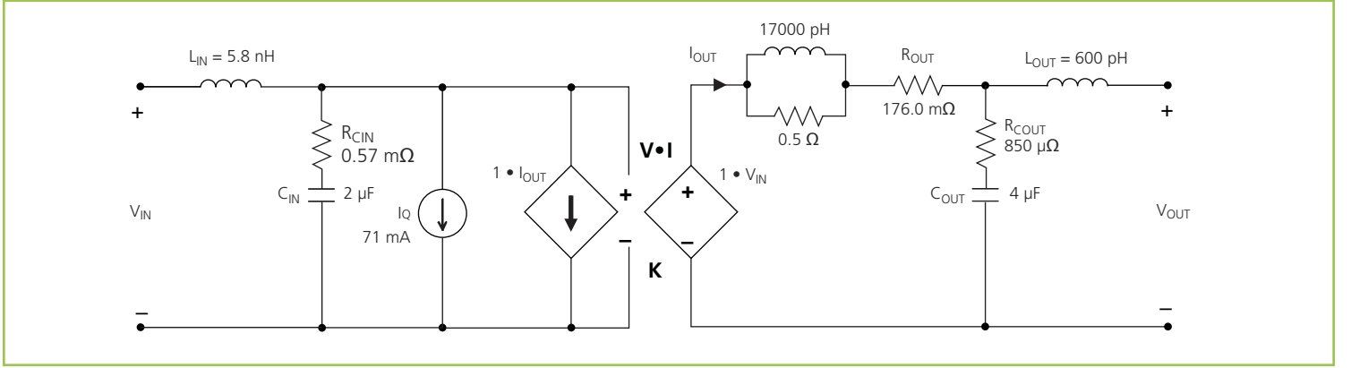
Figure 13 — VI Chip® module AC model
