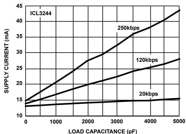
FIGURE 21. SUPPLY CURRENT vs LOAD CAPACITANCE WHEN TRANSMITTING DATA
