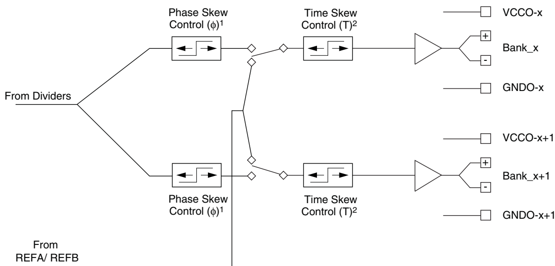
Figure 21. ispClock5400D Output Group and Skew Control
