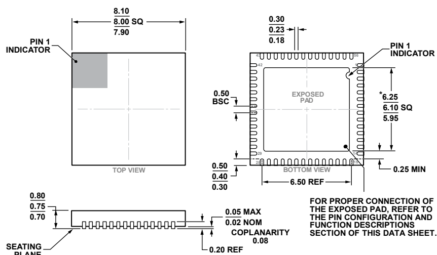
Figure 96. 56-Lead Lead Frame Chip Scale Package [LFCSP]
