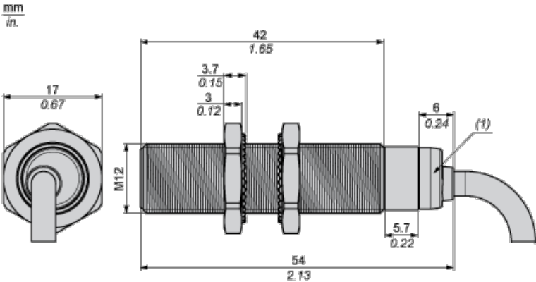
(1) LED
