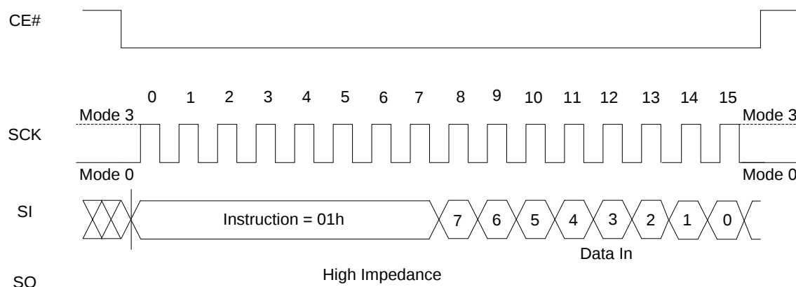
Figure 8.26 Write Status Register Sequence
