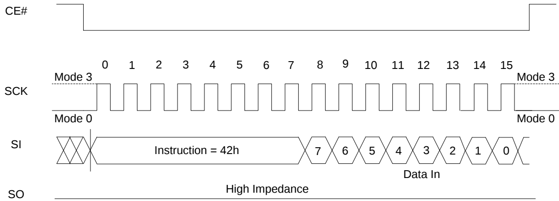
Figure 8.30 Write Function Register Sequence
