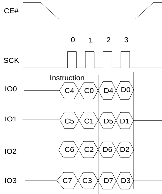
Figure 8.31 WRFR COMMAND (WRITE Function REGISTER) OPERATION (QPI)
