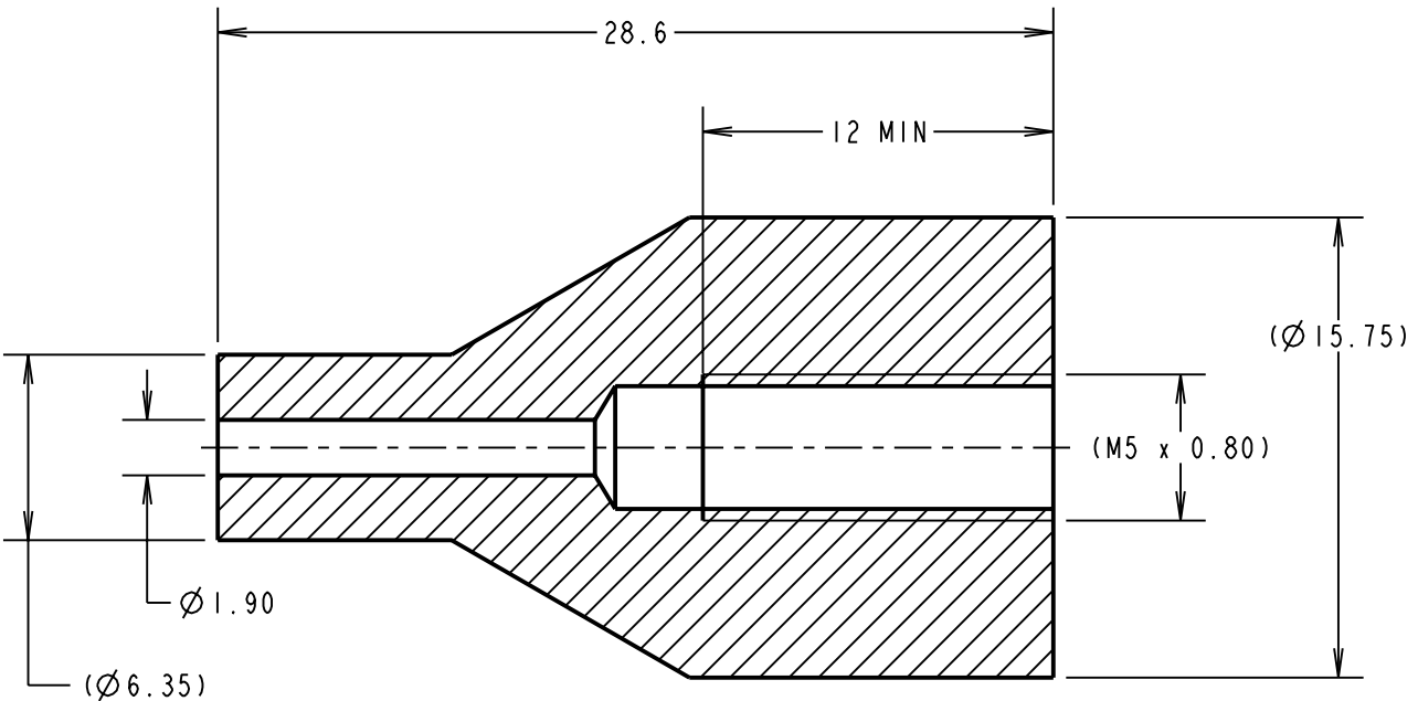
Z10000-00 BOTTOM TOOL PART MACHINED BLANK
