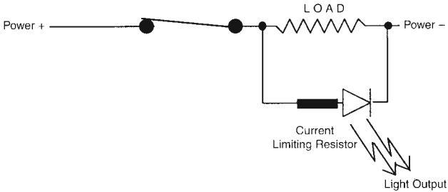
Figure 19. Wiring Diagram 4
