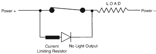
Figure 17. Wiring Diagram 2
