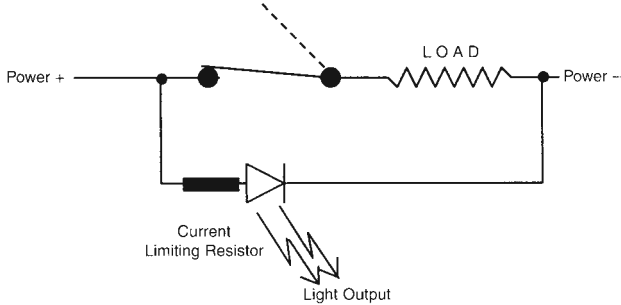
Figure 18. Wiring Diagram 3
