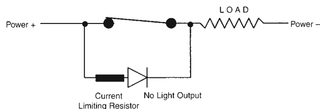
Figure 17. Wiring Diagram 2
