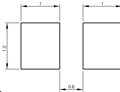
Recommended solder pad Footprint
