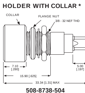
HOLDER WITH COLLAR *
