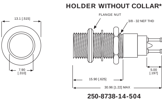
HOLDER WITHOUT COLLAR*
