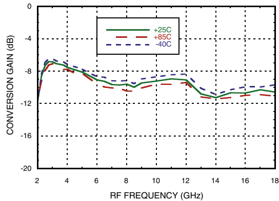
Conversion Gain vs. Temperature, IF= 100 MHz, LO= 13dBm
