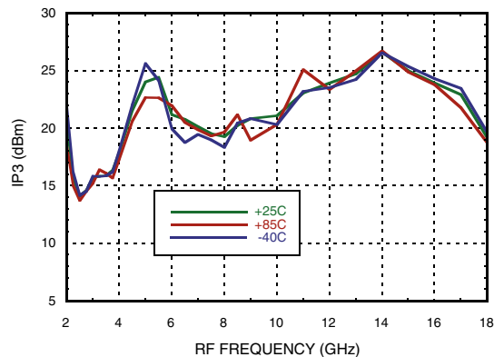
Input IP3 vs. Temperature, IF= 100 MHz, LO= 13dBm
